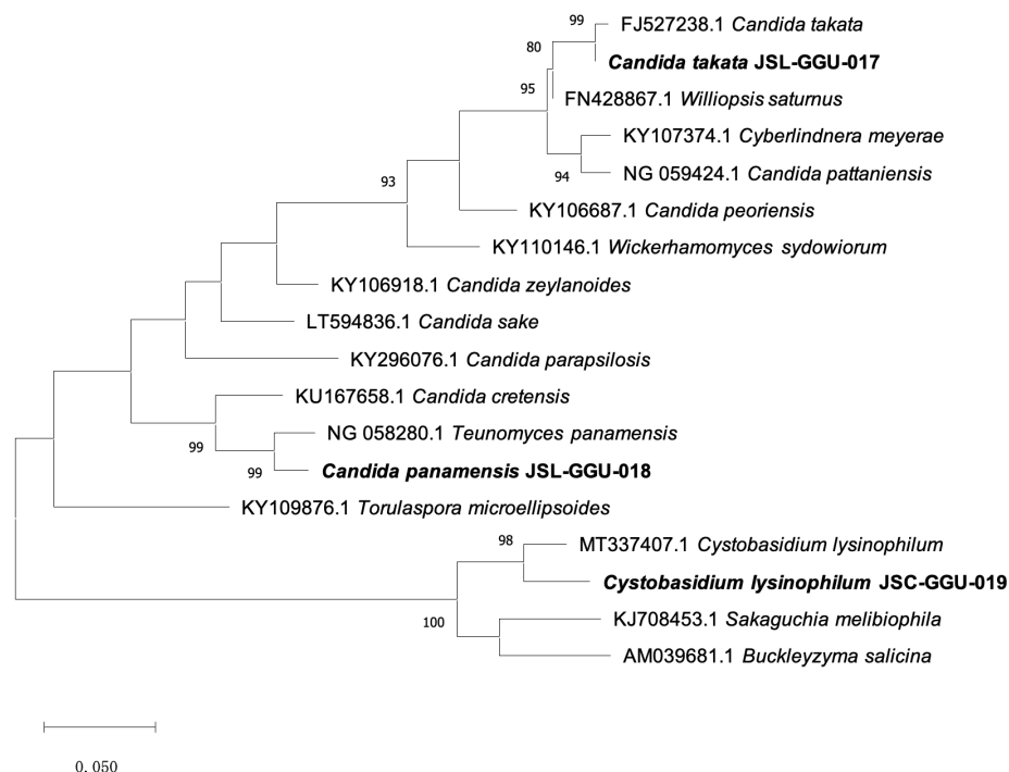
Fig. 2. Phylogenetic tree of the unrecorded yeasts isolated from waters and soils in Jangtaesan and Jangseonchon (RV), based on the nucleotide sequences of large subunit 26S ribosomal DNA D1/D2 region. The tree was generated by the Maximum-likelihood method, using MEGA-X (Glen Stecher, Koichiro Tamura, and Sudhir Kumar (2020) Molecular Evolutionary Genetics Analysis (MEGA) for macOS. Molecular Biology and Evolution 37:1237-1239). Bold type: Candida takata JSL-GGU-017, Candida panamensis JSL-GGU-018 and Cystobasidium lysinophilum JSC-GGU-019 are unrecorded yeasts.
