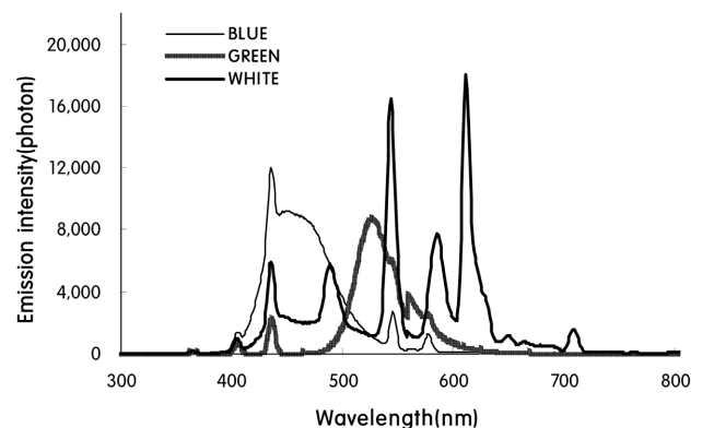
Fig. 1. Transmission light spectra of three light sources.
