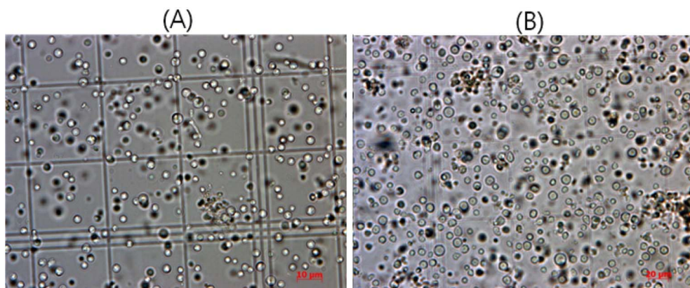
Fig. 1. Effect of cellulase enzymes to release protoplast from Flammulina velutipes . (A), yatalase+cellulase onozuka R-10; (B), Glucanex R 200G+cellulase onozuka R-10. The concentration of protoplasts was calculated 2 \times 10^7 ml -1 and 4 \times 10^7 ml -1 using haemocytometer, respectively.
