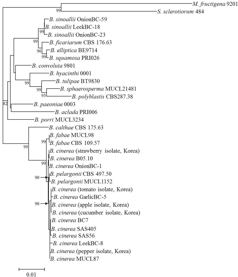
Fig. 3. Phylogenetic analysis constructed by the neighbor-joining method based on combined RPB2 , HSP60 , G3PDH sequence data. Monilinia fructigena and Sclerotinia sclerotiorum were used the outgroup. Numbers above the branches represent the bootstrap values obtained for 100 replicates (smaller than 80 values were not shown). The bar represents a phylogenetic distance of 0.01%.
