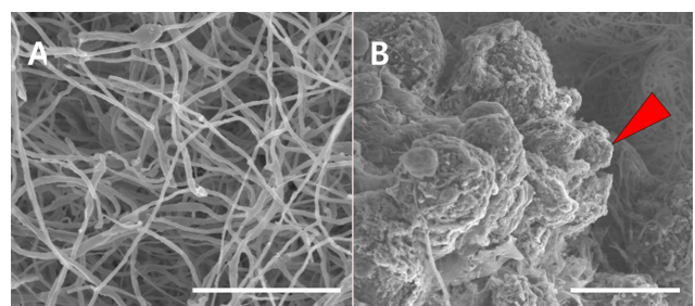
Fig. 3. SEM images of DUCC5000. A: Mycelia 14 days after the growth on PDA. Bar: 100 \mu m. B: Conidiomata observed 35 days after the growth on PDA. Bar: 200 \mu m. Arrow indicates an opened hole.
