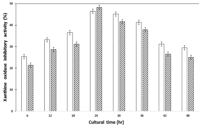
Fig. 1. Effect of cultural times of Kuraishia capsulata UL40-2(□) and Sporobolomyces ruberrimus 121-Z-3(▨) on the production of xanthine oxidase inhibitor.
