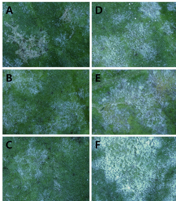
Fig. 3. Comparison of inhibition of mycelium growth by treatment with antagonistic bacterial cell suspension (A, Bacillus sp. M9; B, Bacillus sp. M70; C, Bacillus sp. M99-1; D, commercial goods-1; E, commercial goods-2; F, control) on the colonized leaf disk with mycelium and spores of melon powdery mildew. Antagonistic bacteria ( 1 \times 10^8 CFU/mL) were sprayed onto whole leaf disk. The degree of growth of the mycelium was measured 5 days after treatment, and the photographs were taken under stereo microscopy ( 10\times ).
