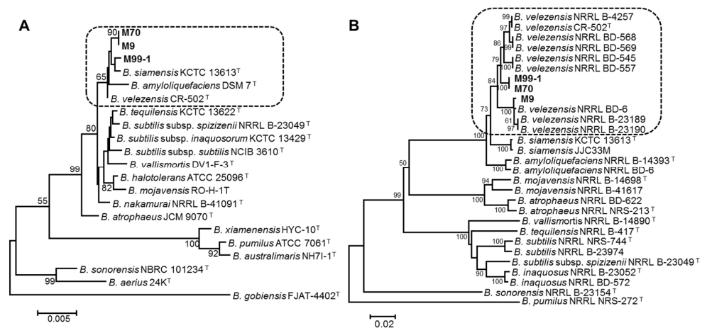
Fig. 1. Neighbor joining trees inferred from 16S rDNA (A) and gyrase subunit A ( gyrA ) (B) gene sequences of Bacillus subtilis species complex. Bootstrap scores > 50 are presented at the nodes. The scale bar indicates the number of nucleotide substitutions per site. The selected antagonistic bacteria are indicated in bold.
