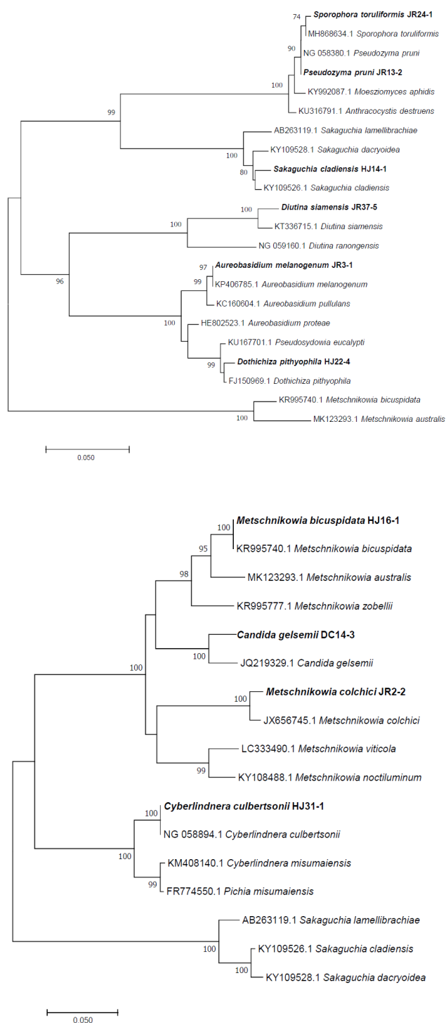
Fig. 1. Phylogenetic tree of the unrecorded yeasts isolated from Hajodae and Gyungpodae Beaches in Korea, based on the nucleotide sequences of D1/D2 region of 26S ribosomal. The tree was generated by the neighbor-joining method, using MEGA7.
