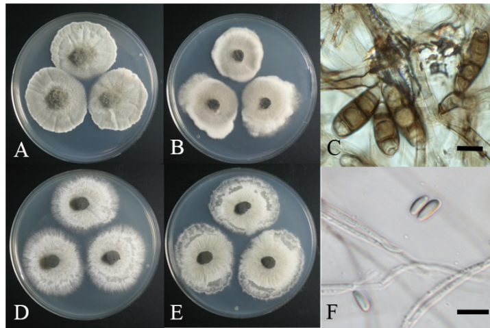
Fig. 1. Colonies of strain 18S001 ( Curvularia protuberata ) grown for 7 days on PDA (A) and MEA (B), C, conidia; D&E, colonies of strain 18S002 ( Didymella anserina ) grown for 7 days on PDA (D) and MEA (E); F, conidia. (scale bars = 10 \mu\text{m} ). PDA, potato dextrose agar; MEA, malt extract agar.
