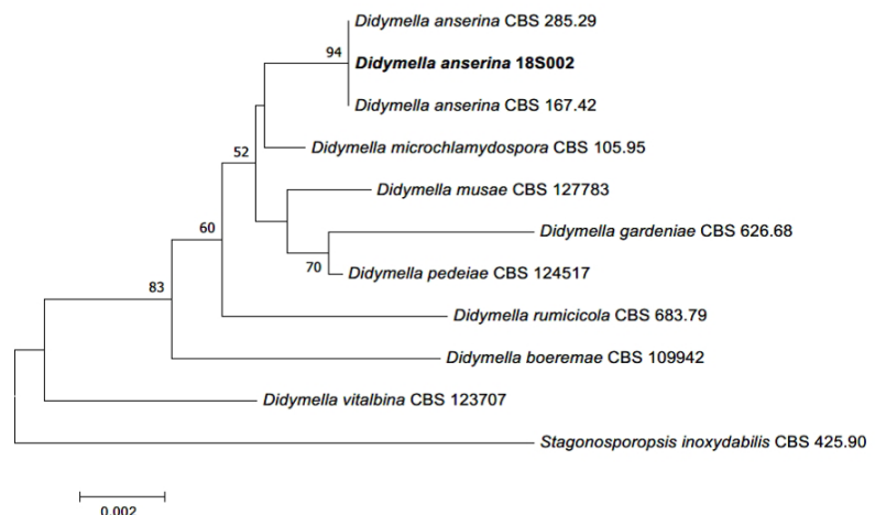
Fig. 3. Neighbor-joining phylogenetic tree based on a concatenated alignment of internal transcribed spacer (ITS) and large subunit (LSU) sequences. Stagonosporopsis inoxydabilis was used as an outgroup. Numbers on branches indicate bootstrap values (1,000 replicates). Fungal strain isolated in this study is in bold.
