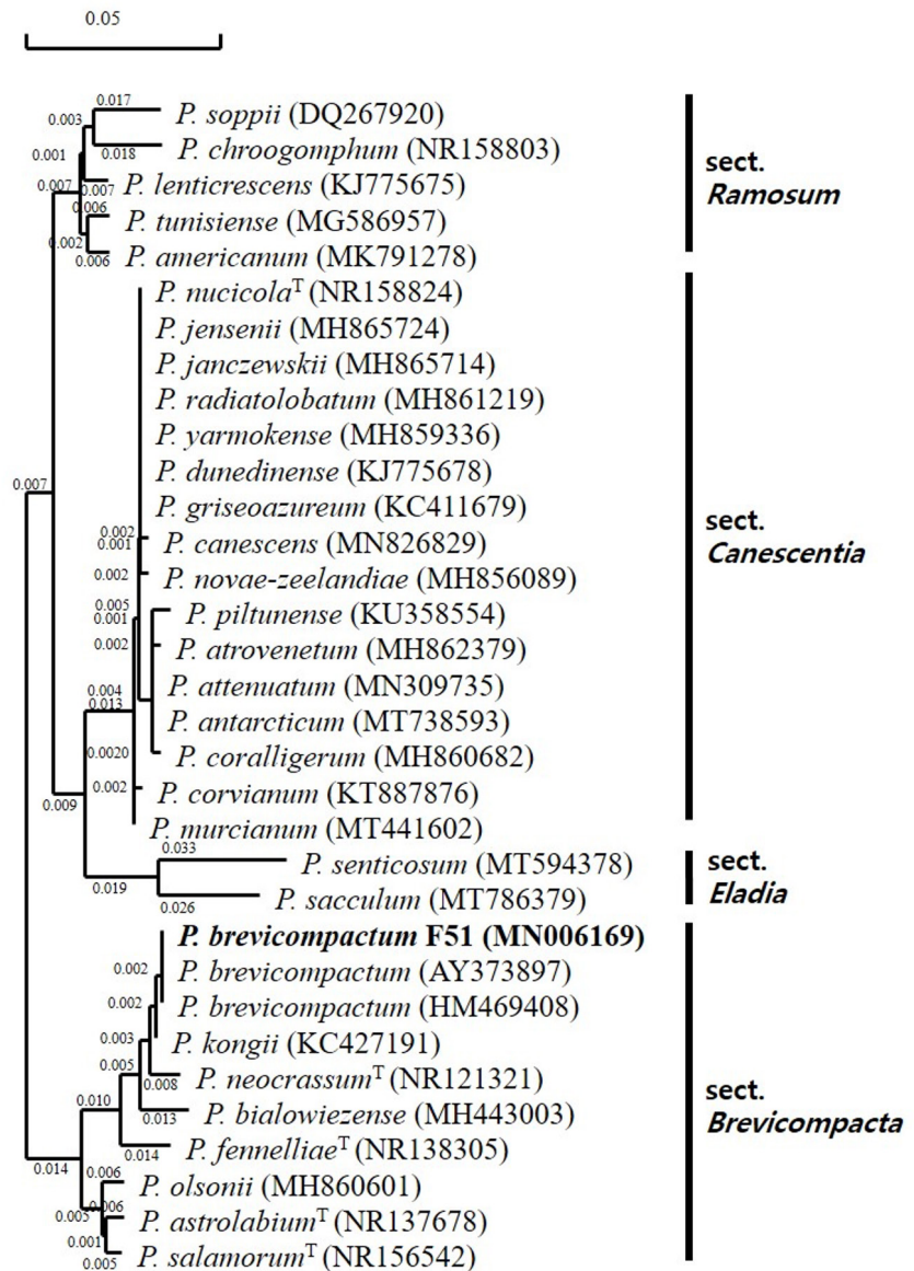
Fig. 3. Phylogenetic tree constructed by the neighbor-joining method, comparing the internal transcribed spacers(ITS) sequences of the presnet isolated strain with those of other Penicillium species from GenBank. Branch lengths are proportional to phylogenetic distance. The scale bar represents genetic distance. T = type strain. The name in bold type is the isolated strain described in this study.
