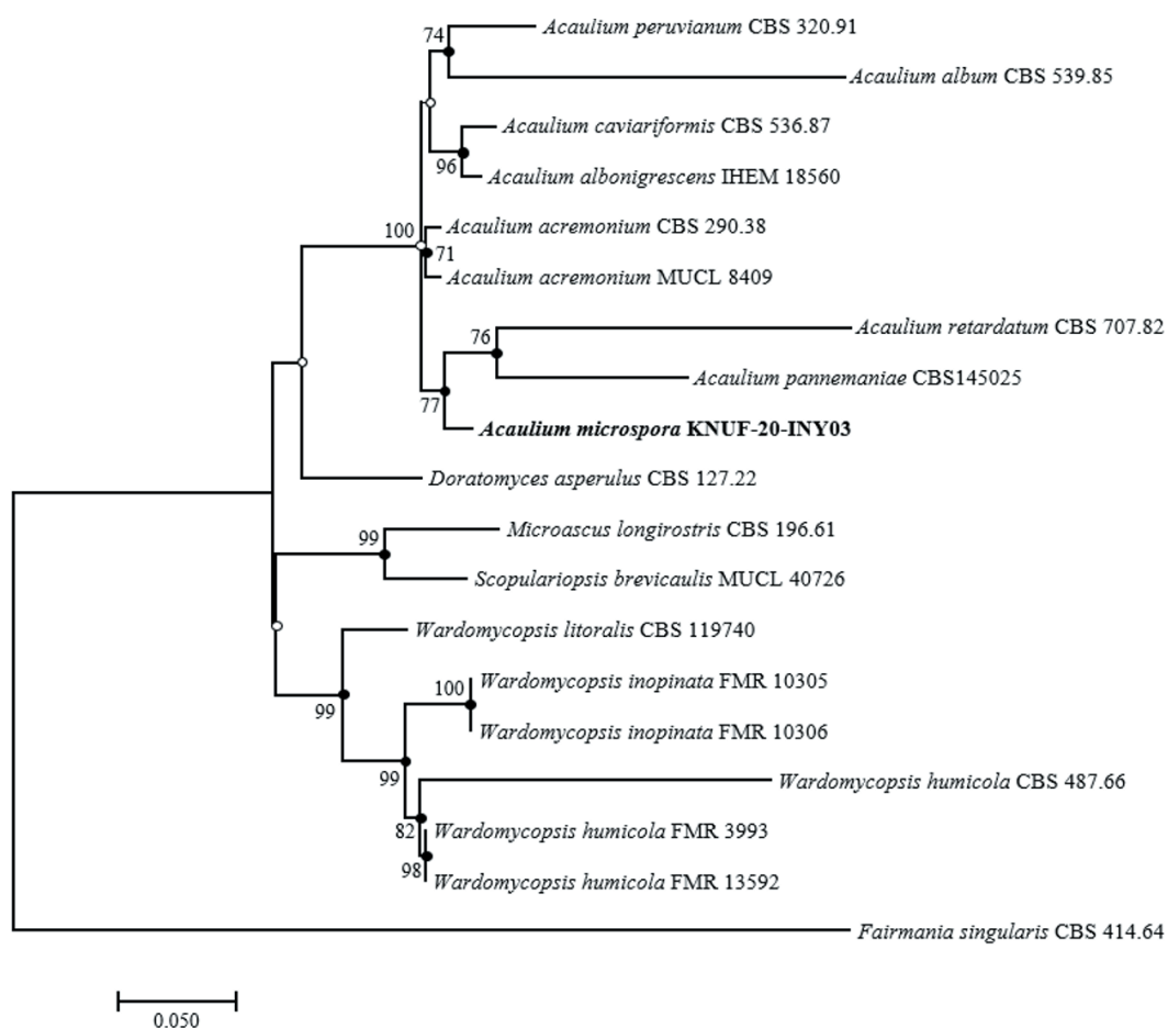
Fig. 2. Maximum-likelihood phylogenetic tree of KNUF-20-INY03 based on the combined sequences internal transcribed spacer (ITS) regions, \beta -tubulin ( \beta -TUB), translation elongation factor 1- \alpha (TEF1- \alpha ) and large subunit of the nuclear ribosomal RNA (LSU), showing the phylogenetic position of novel strain KNUF-20-INY03 among Acaulium spp. and other closely related fungal species. Bootstrap values (based on 1,000 replications) greater than 70% are shown at branch points. Filled circles indicate that the corresponding nodes were also recovered in trees generated using the neighbor-joining and maximum-parsimony algorithms. Open circles indicate that the corresponding nodes were also recovered in the tree generated using the neighbor-joining or maximum-parsimony algorithm. The isolated strain is shown in bold. Fairmania singularis CBS 414.64 was used as an outgroup. Bar, 0.05 substitutions per nucleotide position.
