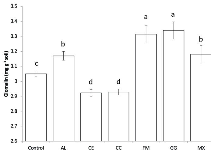
Fig. 2. Total glomalin contents (mg g -1 soil) measured using ELISA (IRSP) in soils after 10 weeks of red pepper growth in fields. A-D: Different letters indicate significant differences at p < 0.05 ( n=6 ) according to LSD test of one-way ANOVA. AL, Acaulospora longula ; CC, Claroidioglomus claroideum ; CE, Claroidioglomus etunicatum ; FM, Funneliformis mosseae ; GG, Gigaspora gigantea ; MX, mixture.
