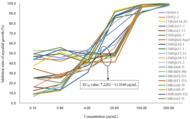
Fig. 3. Baseline of fungicide response resistant to propiconazole on isolates of Fusarium graminearum species complex during 2010-2016 in Jeolla province.
