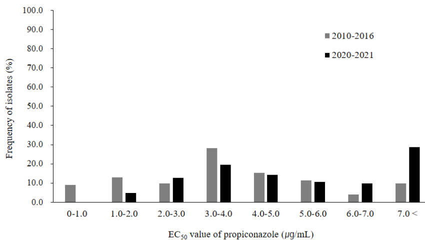
Fig. 2. Frequency distribution of 50% effective concentration ( EC_{50} ) values of Fusarium graminearum species complex isolated from barley and wheat in 2010-2016 and 2020-2021.
