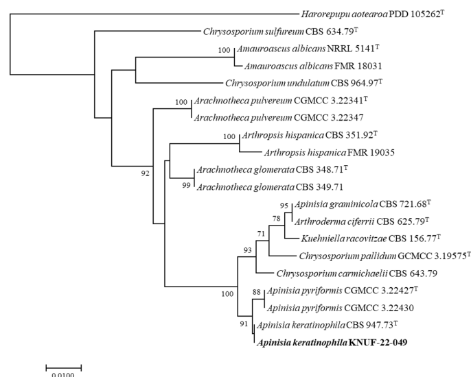
Fig. 3. Neighbor-joining phylogenetic tree based on 28S large subunit of the nrRNA gene (LSU) gene sequences showing the position of Apinisia keratinophila KNUF-22-049 among related strains. Bootstrap values (based on 1,000 replications) greater than 70% are shown at the branch points. The tree was rooted using Harorepupu aotearoa PDD 105262 as the outgroup. The scale bar represents 0.01 substitutions per nucleotide position. ‘T’ indicates type strain.
