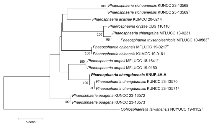
Fig. 3. Maximum-likelihood phylogenetic tree of strain KNUF-4H-A based on the concatenated sequences of internal transcribed spacer (ITS) regions, as well as the large subunit rDNA (LSU) and small subunit rDNA (SSU) genes, showing the phylogenetic position of the new isolate among Phaeosphaeria species. The numbers above the branches represent the bootstrap values (>70%) obtained for 1,000 replicates. The isolated strain is shown in bold. Ophiosphaerella taiwanensis NCYUCC 19-0152 T was used as an outgroup. Bar, 0.005 substitutions per nucleotide position. "T" indicates type strain.
